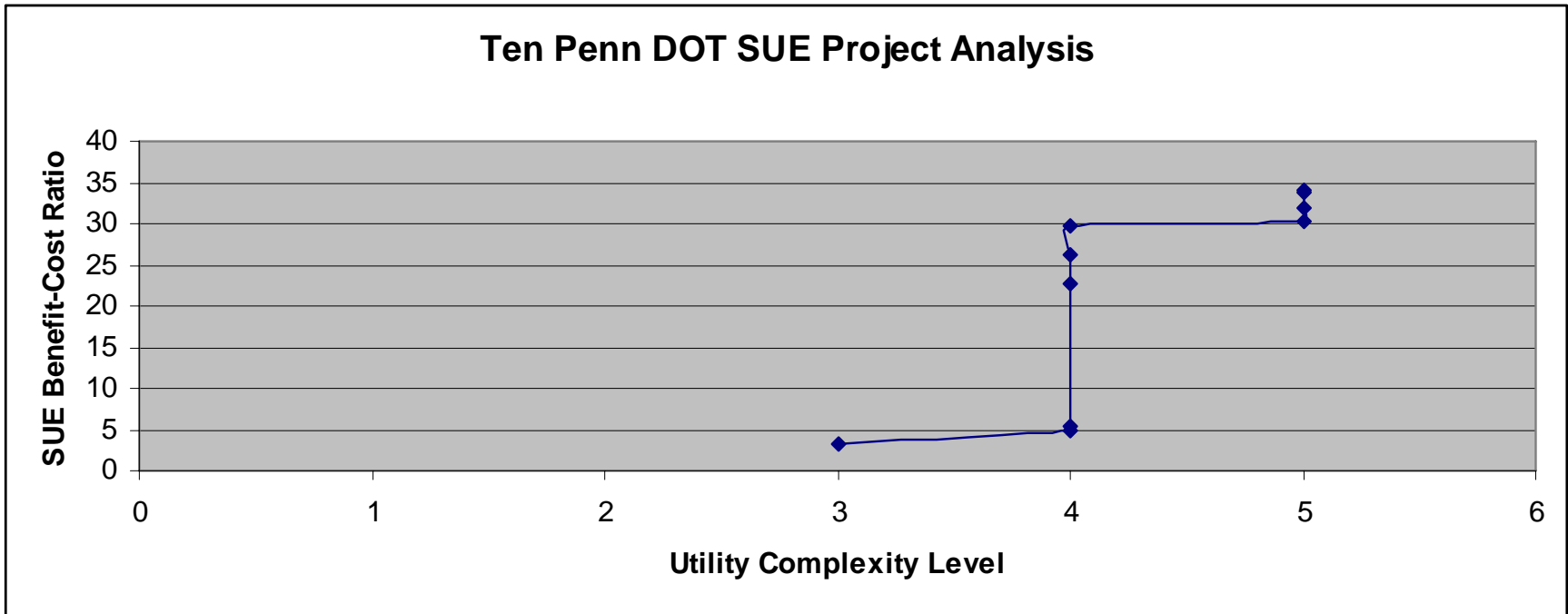
Figure 7-3. SUE Benefit-Cost Ratio vs. Utility Complexity Level Shows Strong Relationship.
