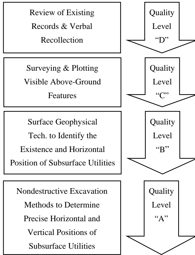
Figure 2-1. Quality Levels of SUE.
