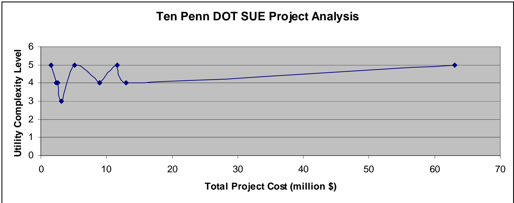
Figure 7-2. Utility Complexity Level vs. Total Project Cost Shows No Relationship.
